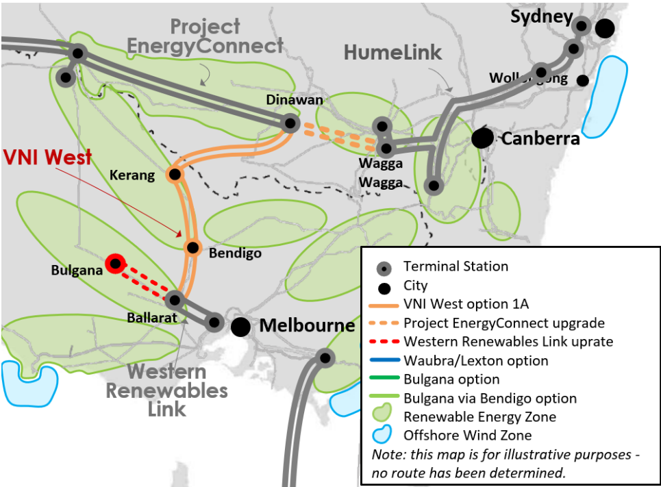
Figure 29 Summary of Option 1A
