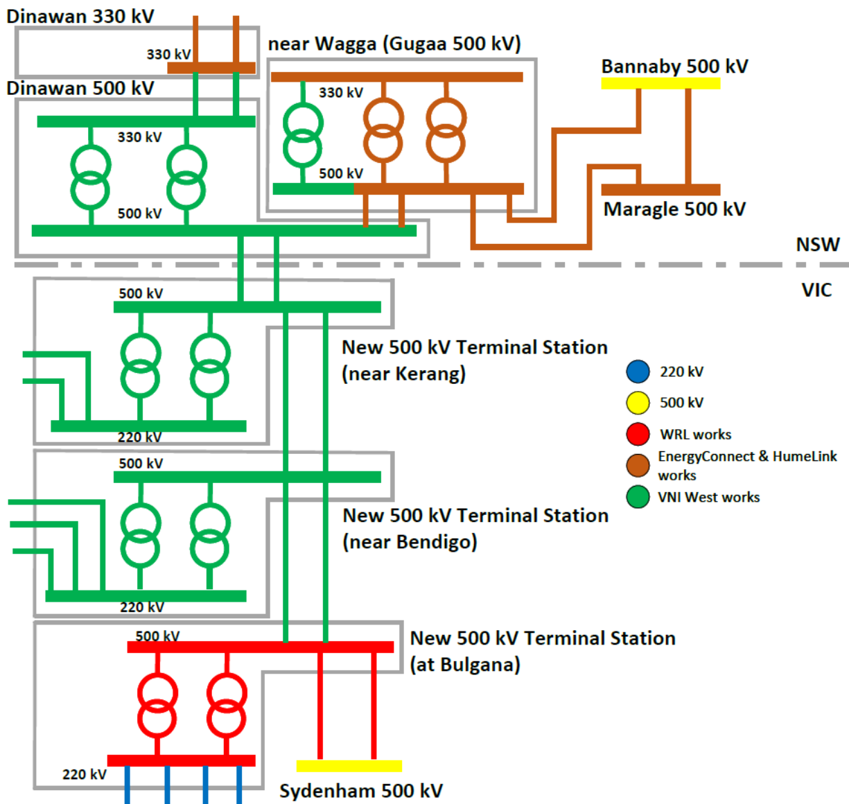
Figure 36 Single-line diagram for Option 4
