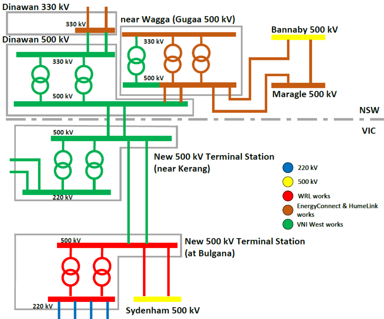
Figure 38 Single-line diagram for Option 5
