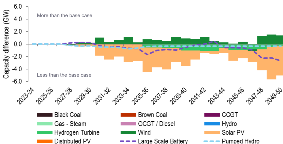
Figure 51 Difference in cumulative capacity built with Option 3A, compared to the base case, under the Hydrogen Superpower scenario
