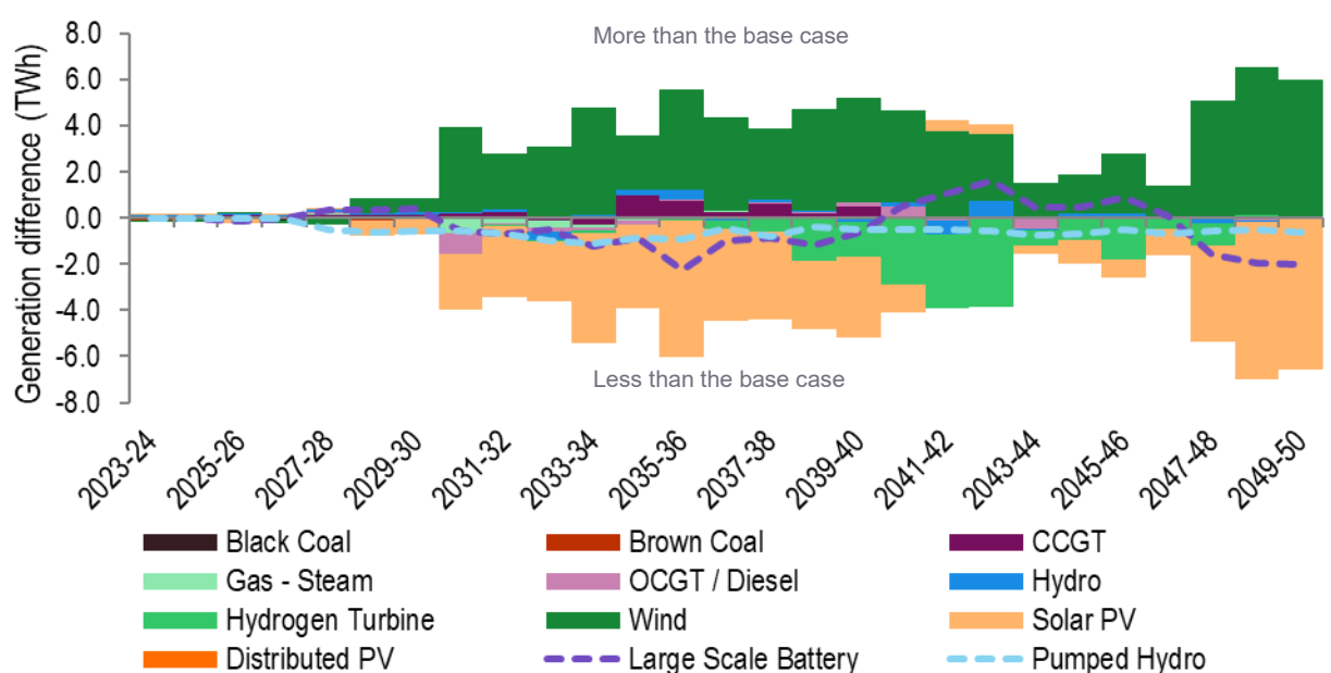
Figure 53 Difference in output with Option 3A, compared to the base case, under the Hydrogen Superpower scenario
