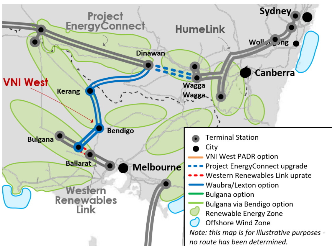
Figure 31 Summary of Option 3
