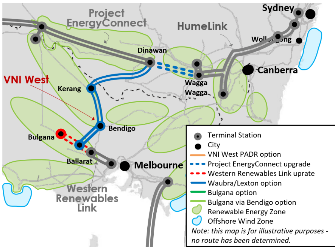
Figure 33 Summary of Option 3A
