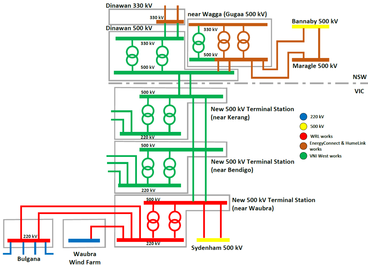
Figure 32 Single-line diagram for Option 3
