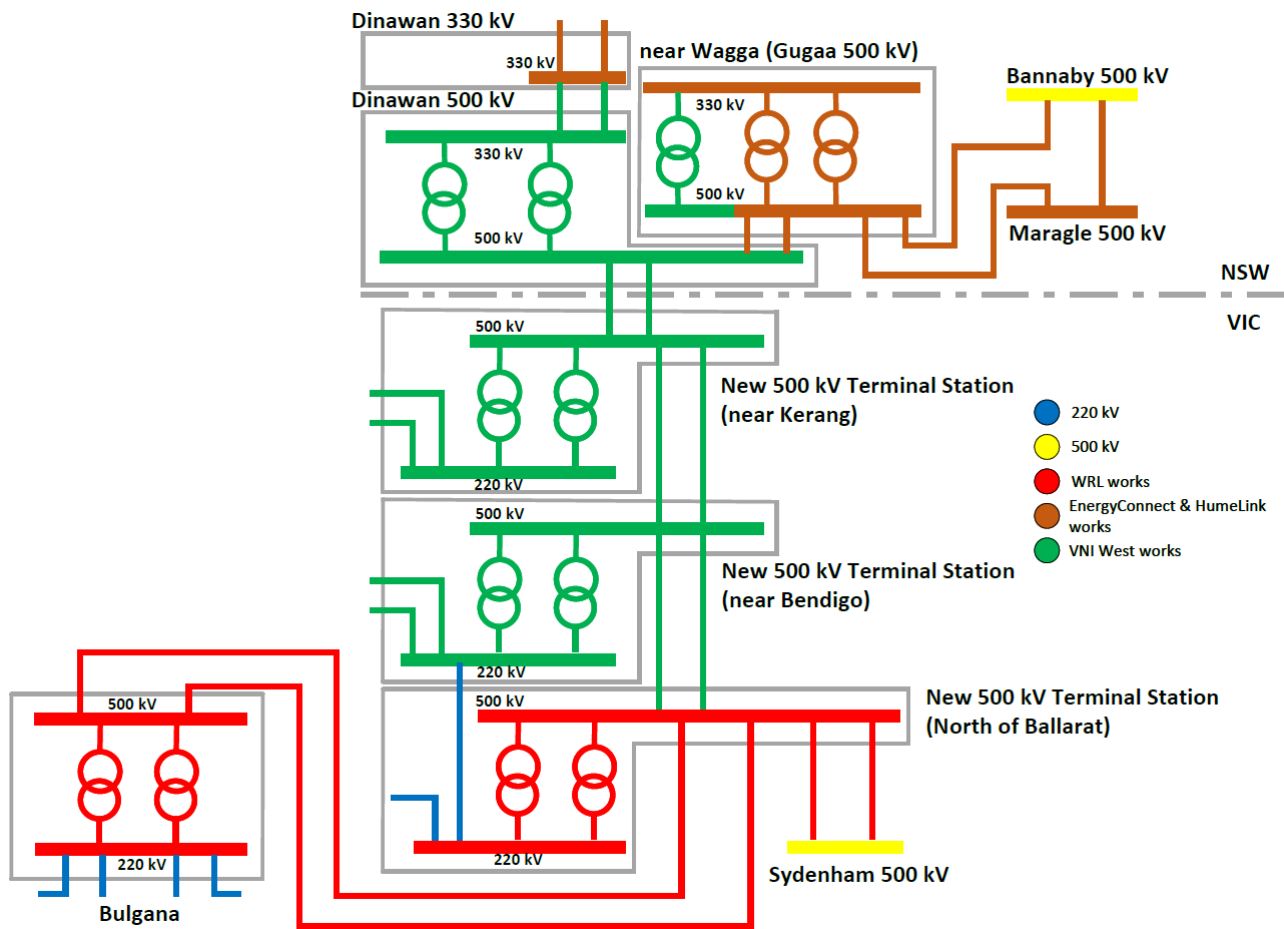
Figure 30 Single-line diagram for Option 1A
