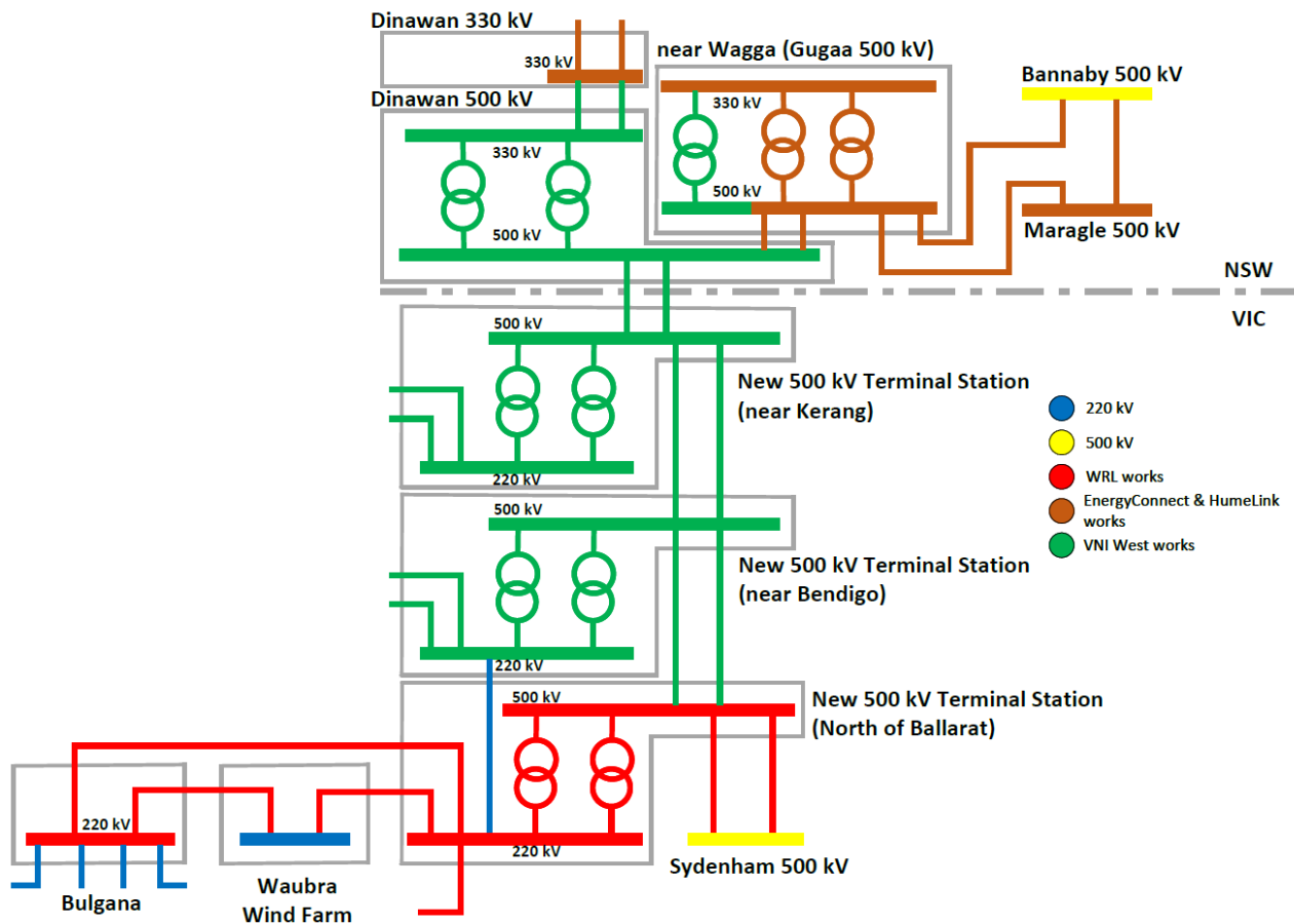
Figure 28 Single-line diagram for Option 1
