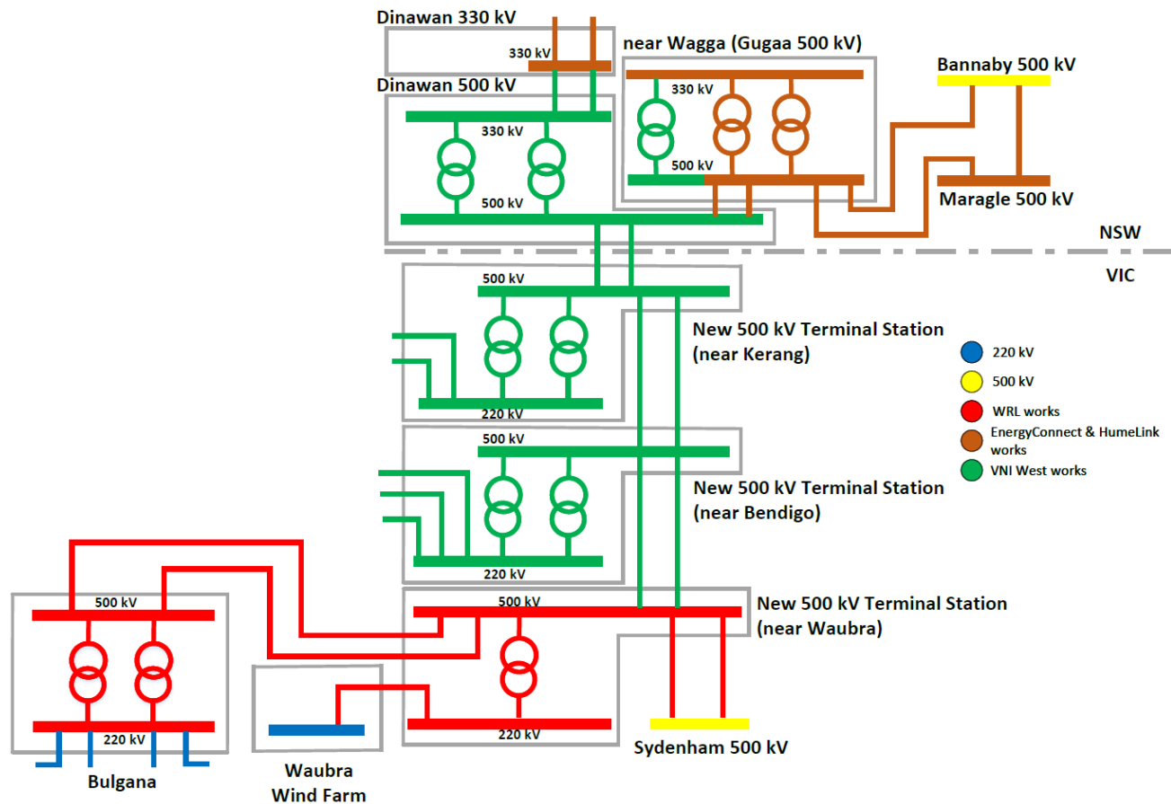
Figure 34 Single-line diagram for Option 3A
