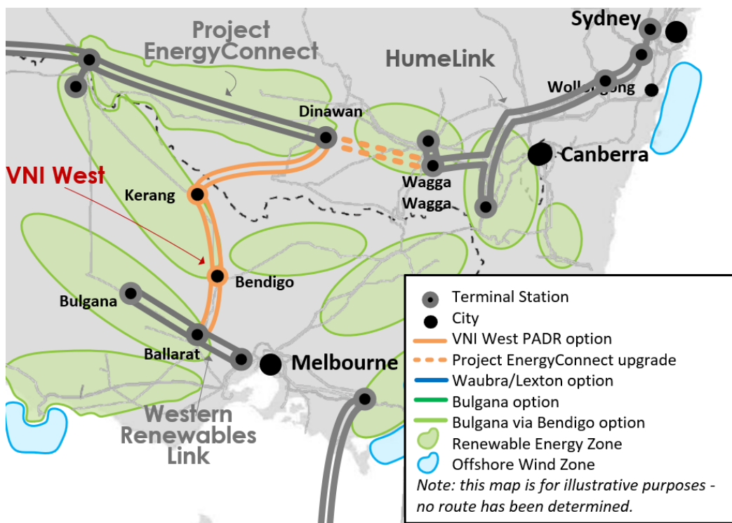
Figure 27 Summary of Option 1
