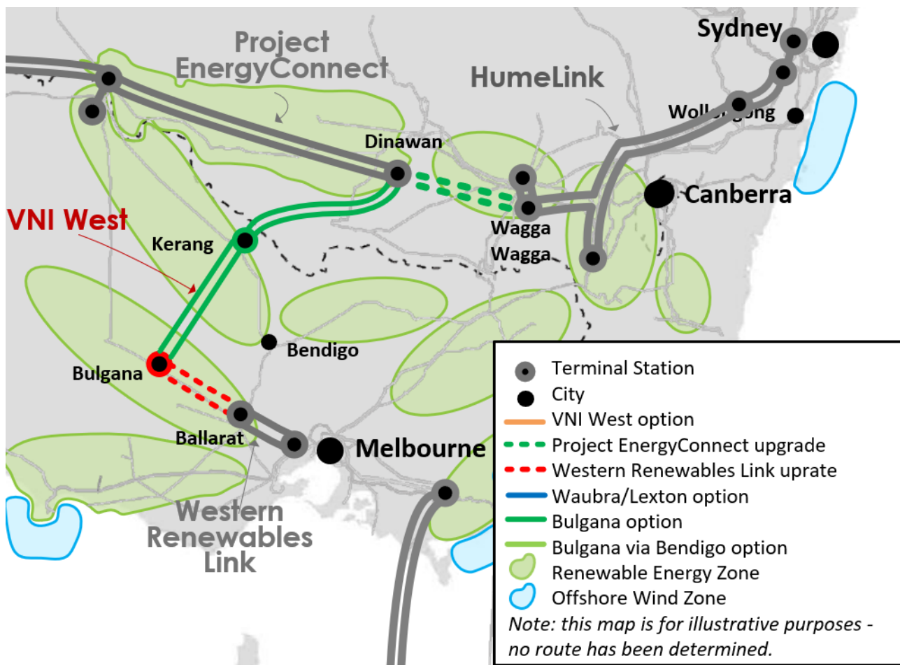
Figure 37 Summary of Option 5
