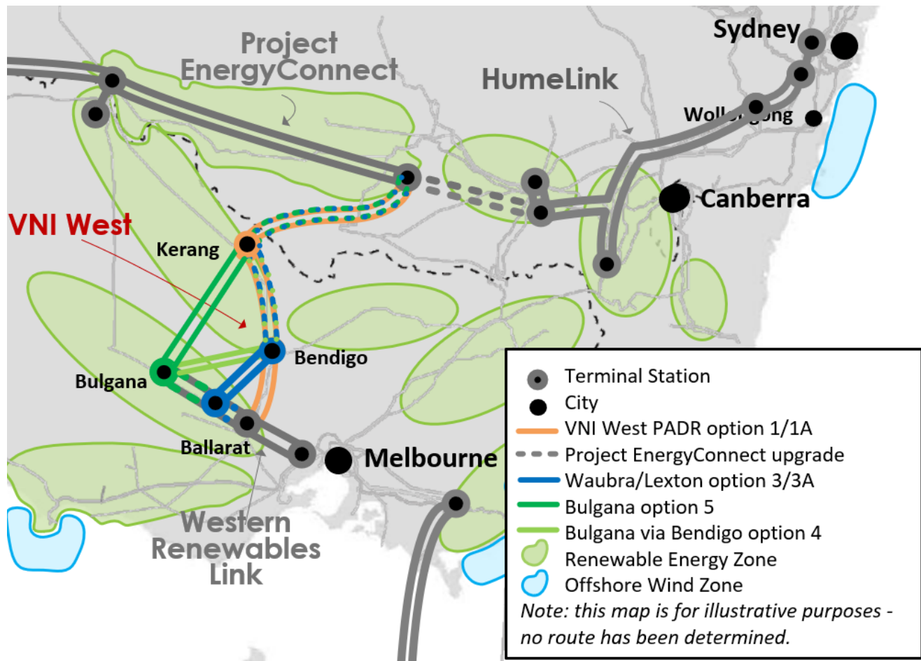
Figure 3 Credible options assessed
