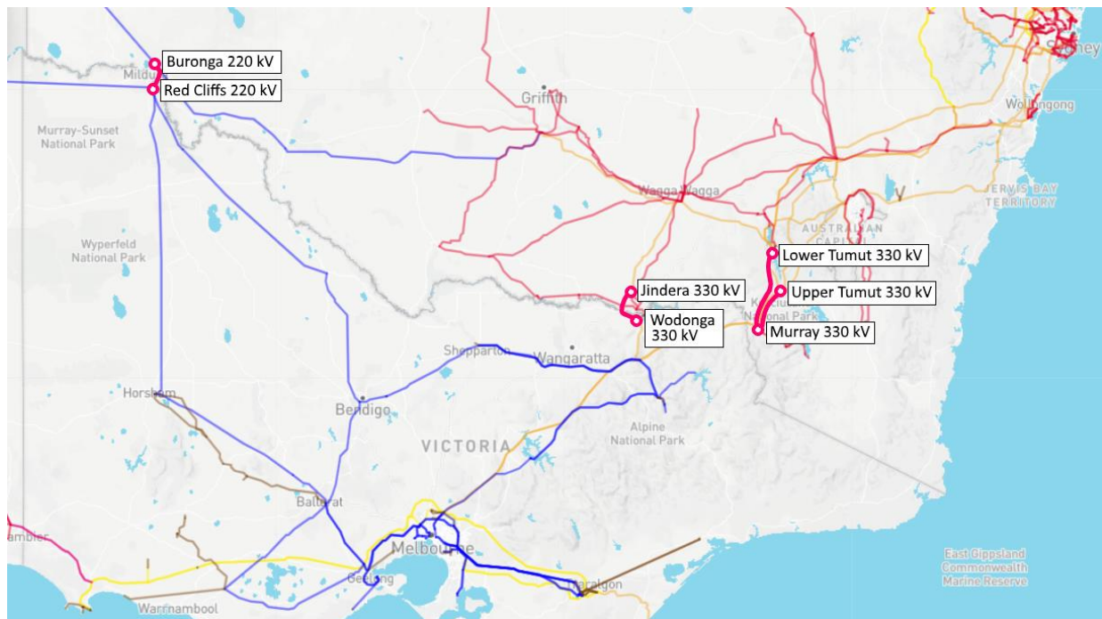
Figure 6 Existing Victoria to New South Wales interconnection routes
