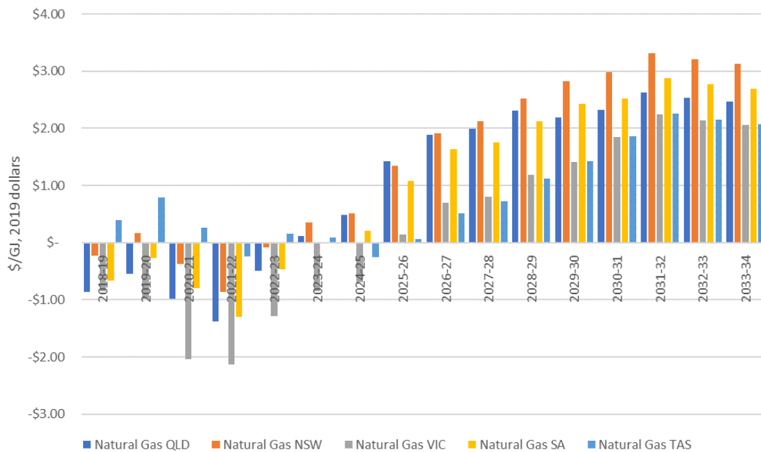
Figure 5 Comparing fuel cost of gas, Neutral scenario
