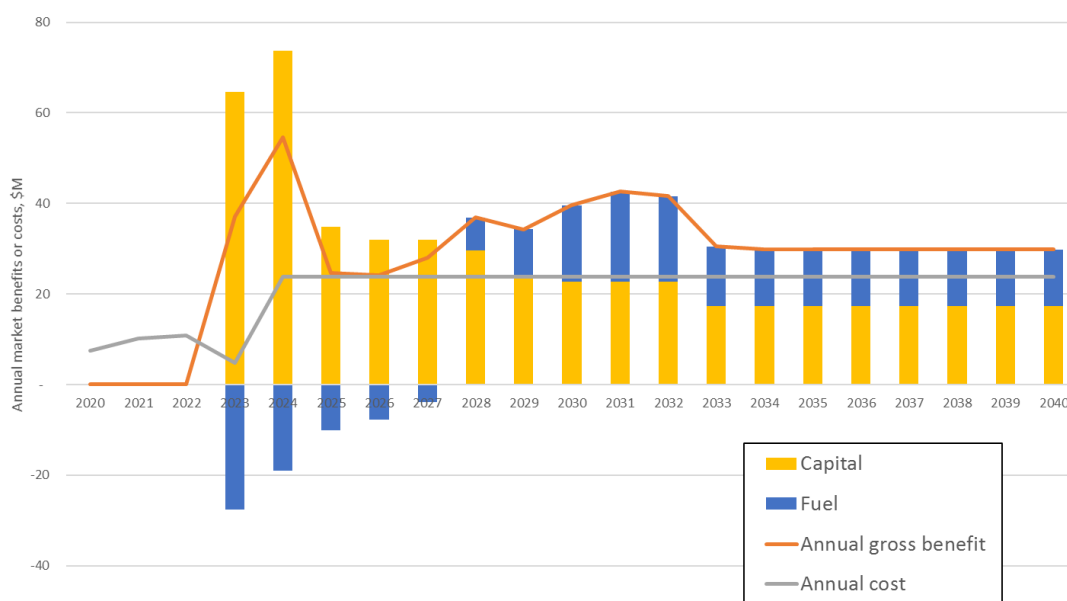
Figure 6 Gross market benefits and annualised costs of Option B3, Neutral scenario
