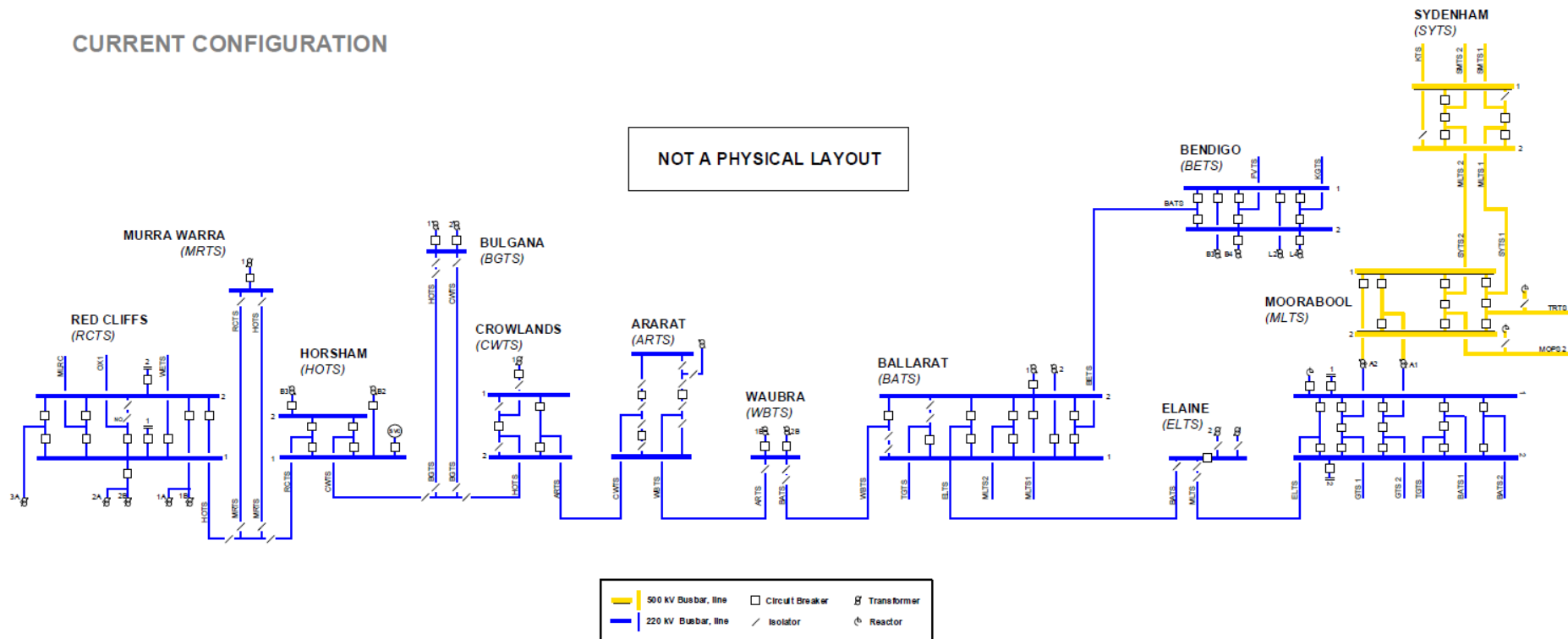
Figure 20 Single line diagram of current network configuration
