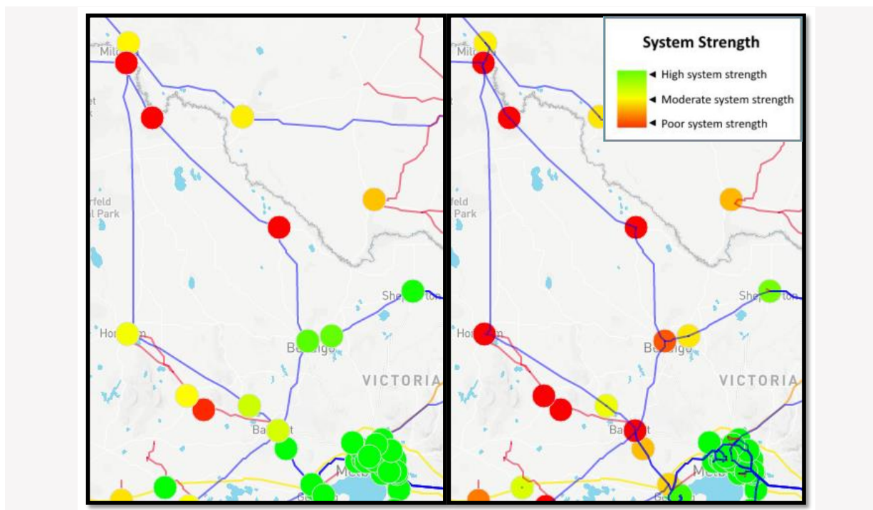
Figure 3 System strength assessment in 2016–17 (left) and 2035–36 (right)
