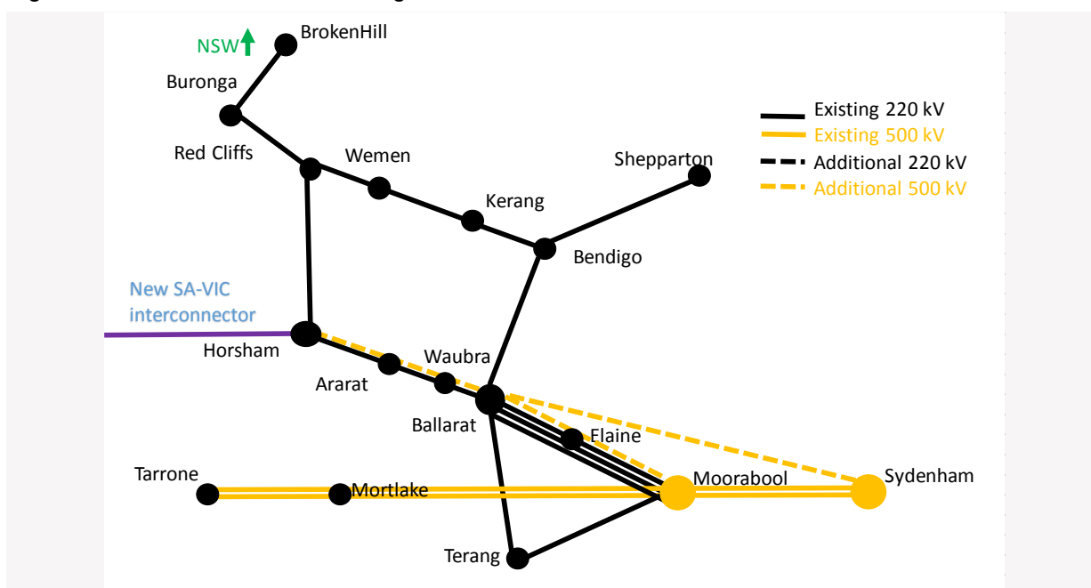
Figure 8 Potential 500 kV network augmentation
