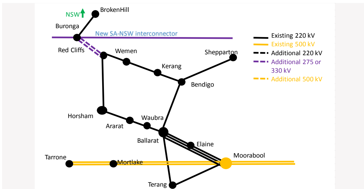
Figure 7 Potential 500 kV network augmentation
