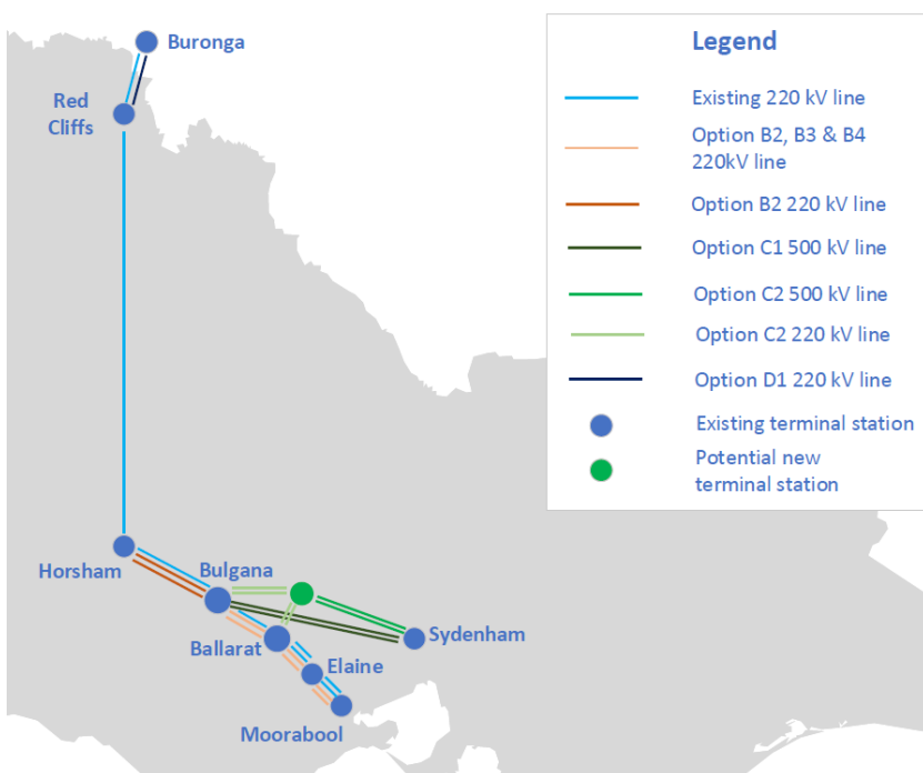
Figure 3 High level overview of major network options
