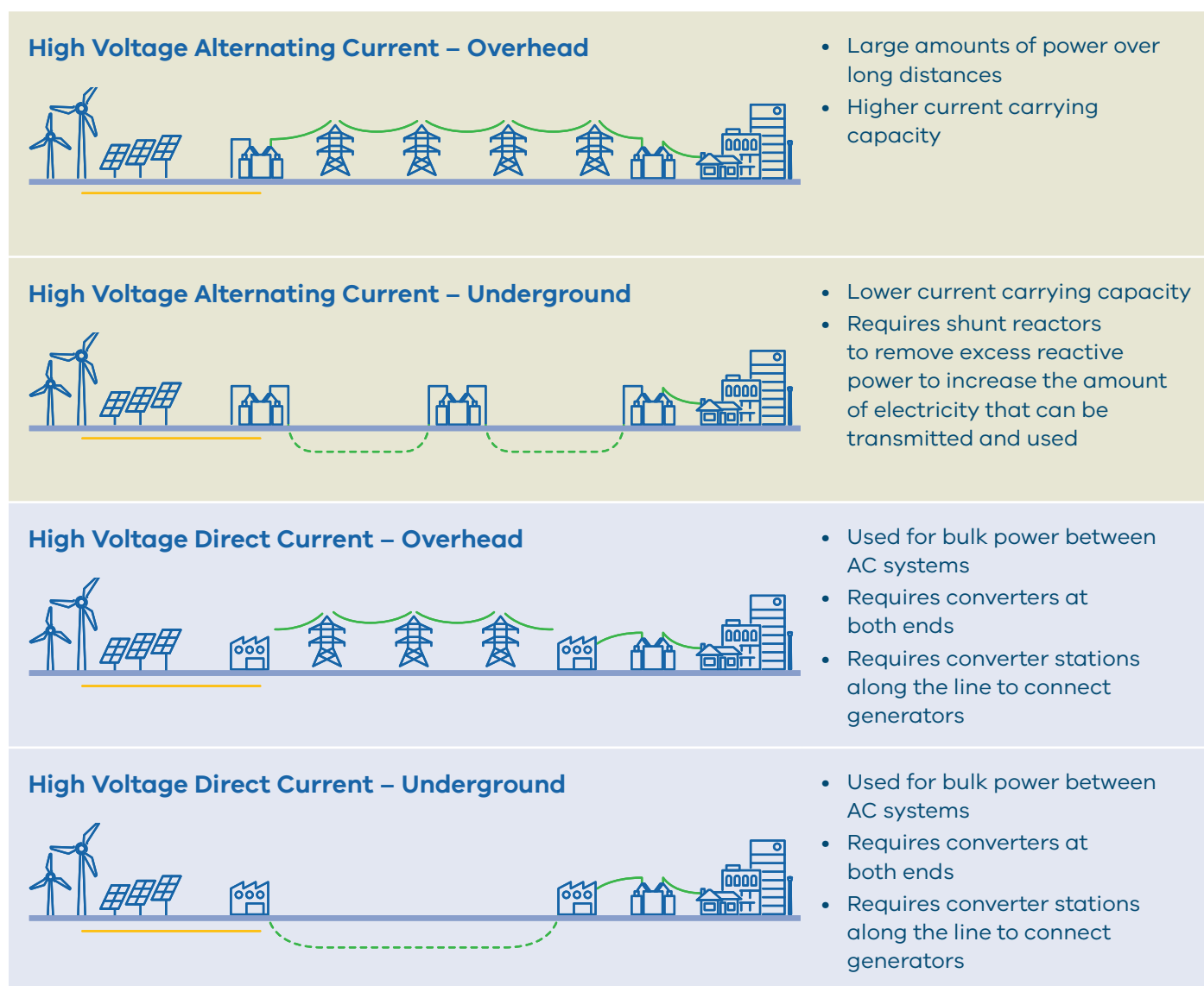
FIGURE 2 Transmission infrastructure types
