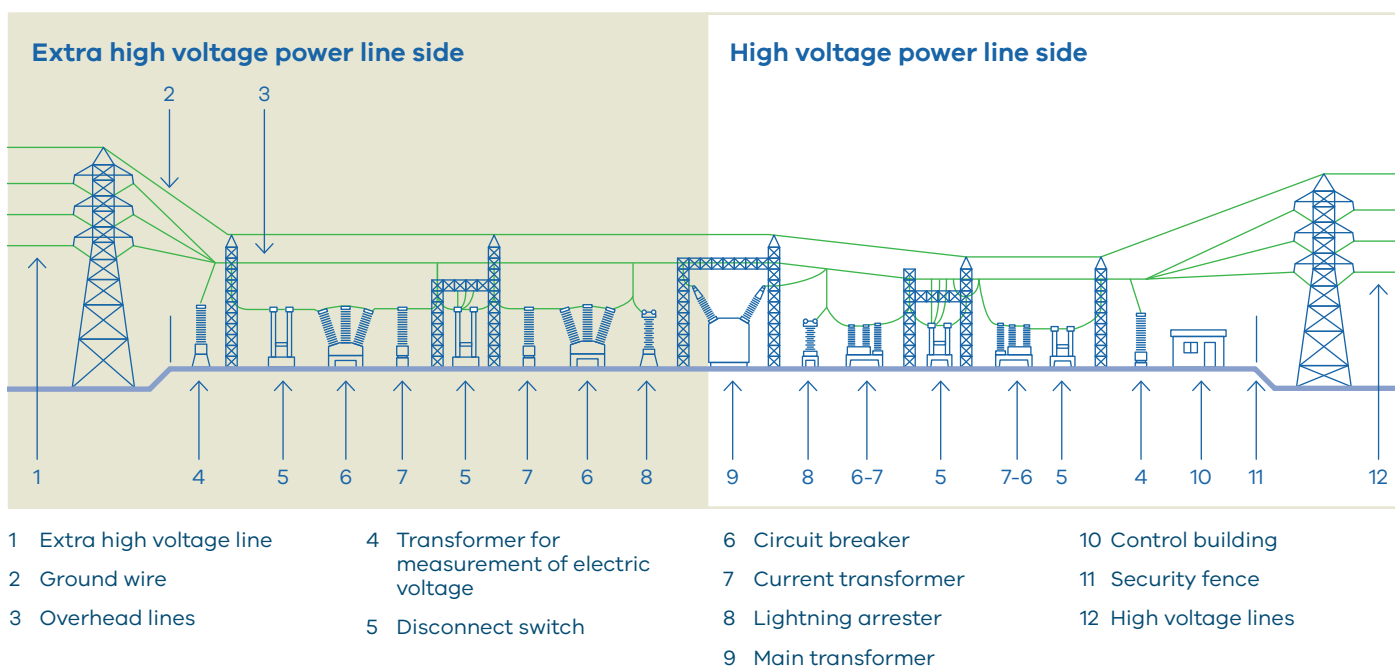
FIGURE 9 Key parts of a terminal station
