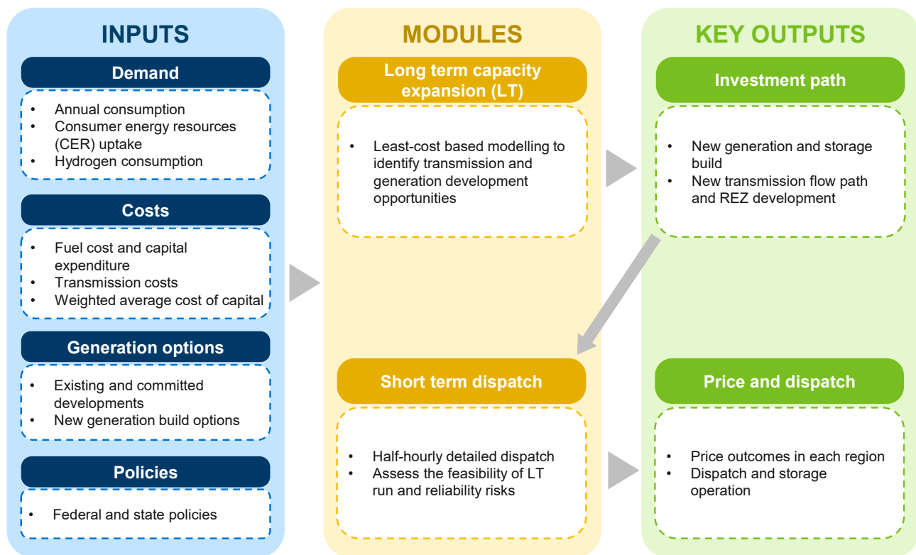
Figure B-2: Energy market modelling process flow
