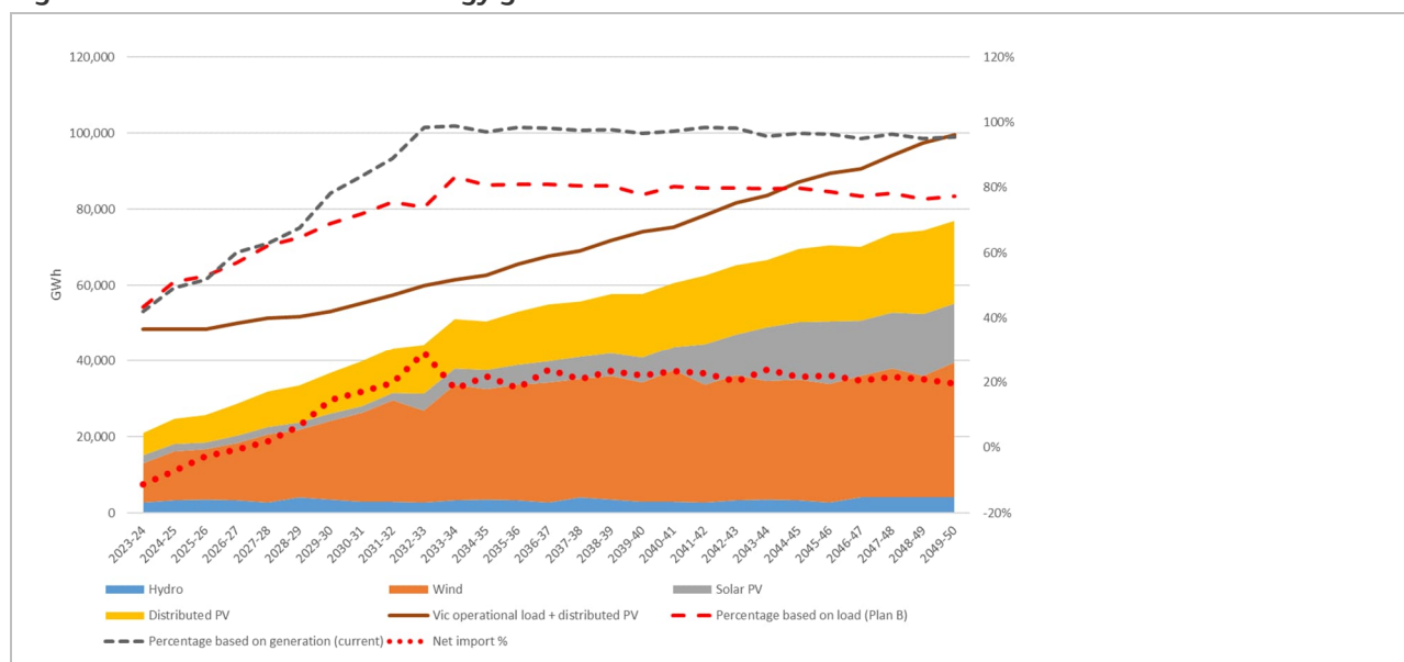
Figure 7. Victorian renewable energy generation with VNIW 51
