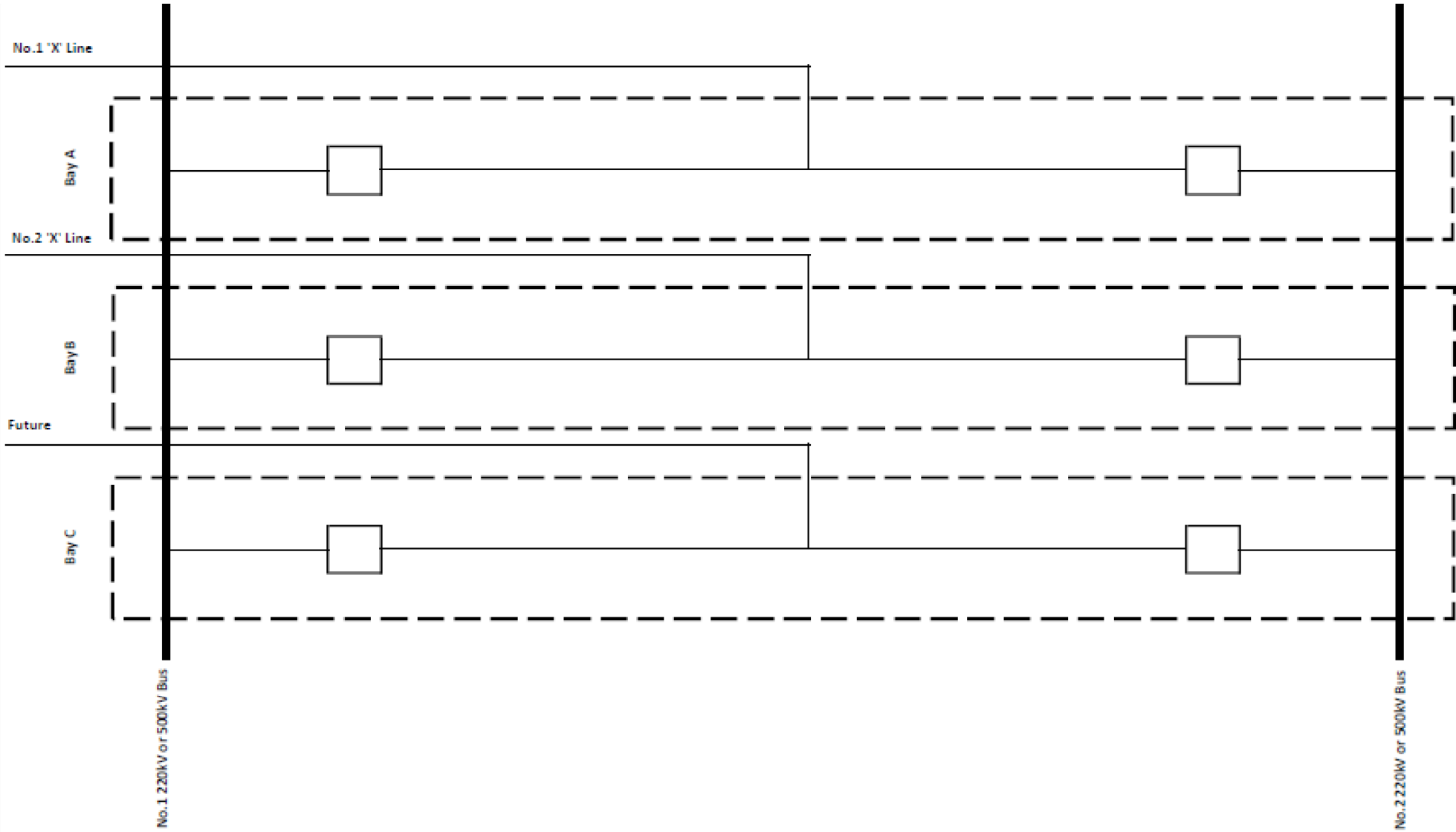
Figure 8: Example of double breaker – double bus arrangement
