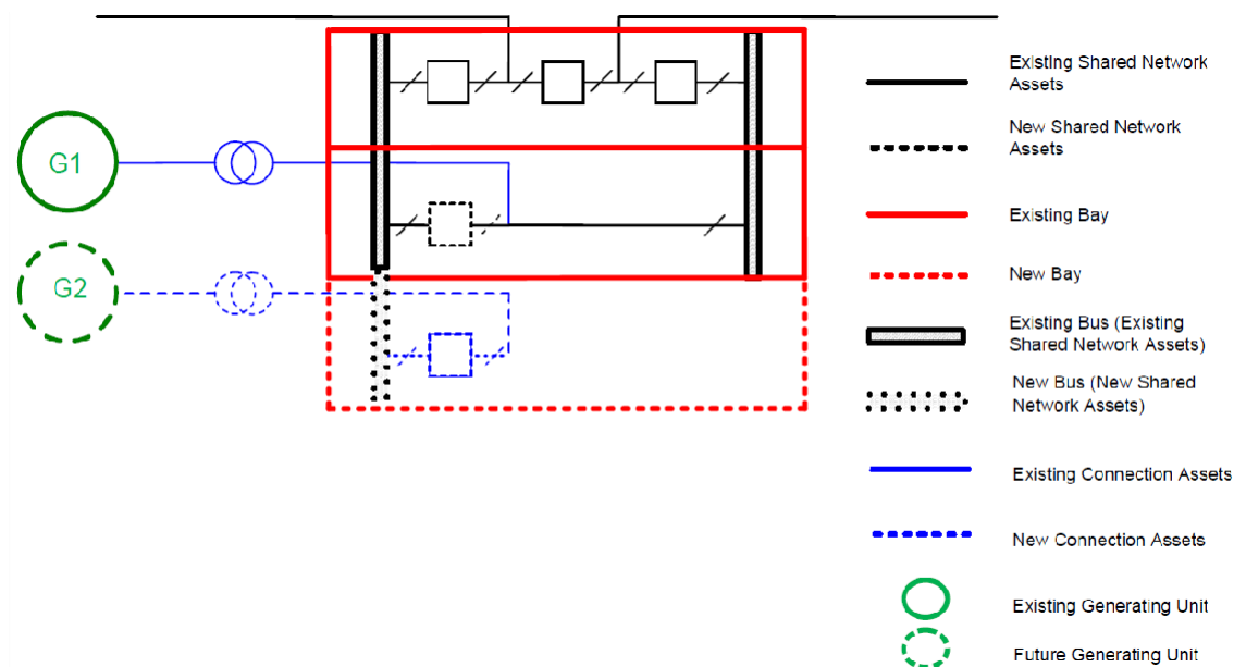
Figure 4: Connection to an existing terminal station (before commissioning of new connection)
