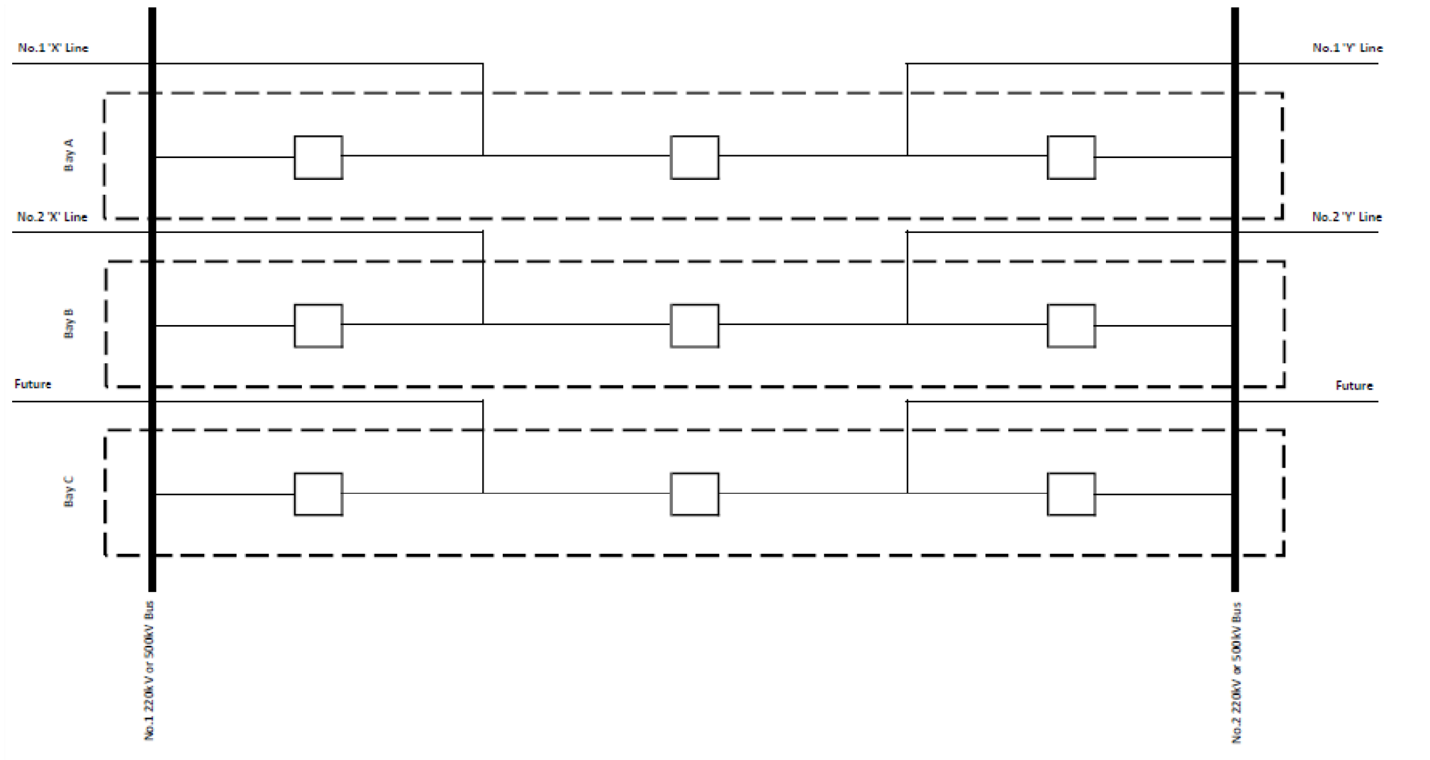
Figure 7: Example of breaker-and-a-half arrangement
